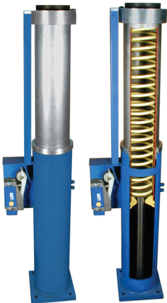
External View of Buffer
