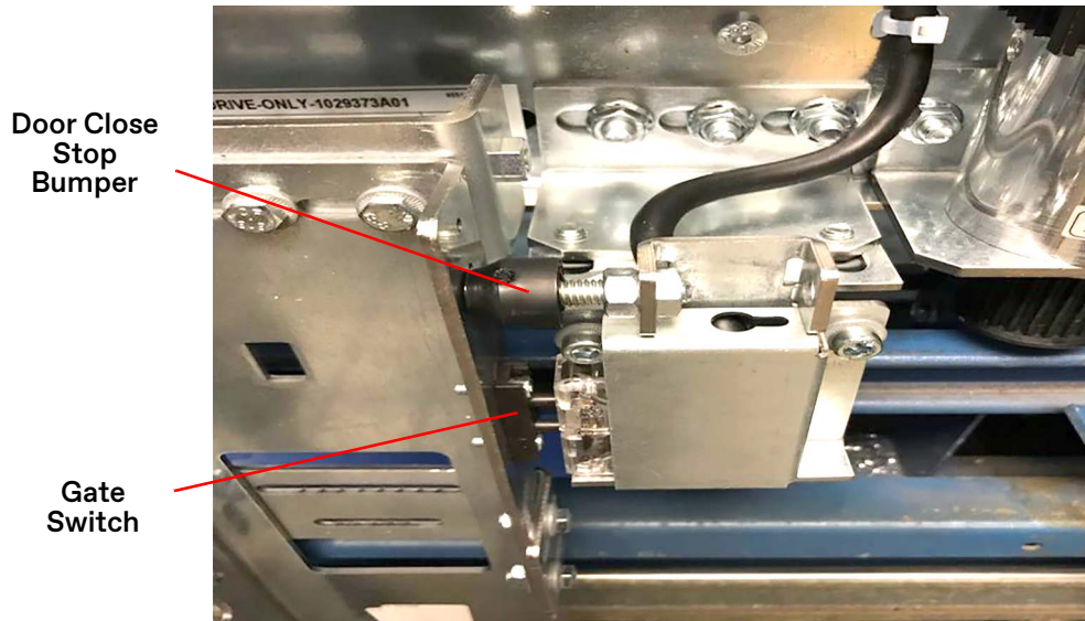
Figure 6 - Adjust Gate Switch and Door Stop Bumper
