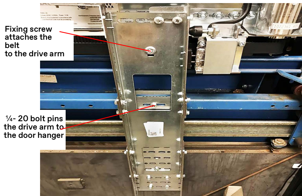
Figure 11 - Pin the Drive Arm/Completed Belt Installation
