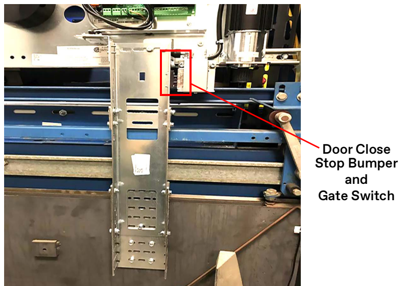
Figure 5 - Install the Drive Arm
