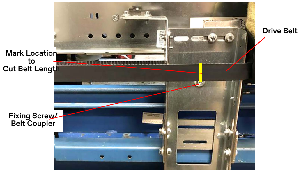
Figure 9 - Drive Belt Installation
