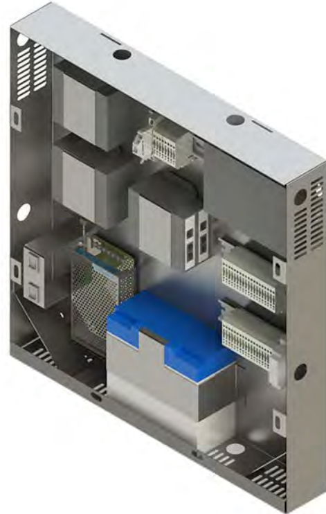
Remote Equipment Box Assembly (2104DN)
