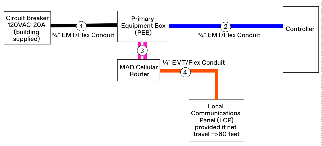
Standard Machine Room
