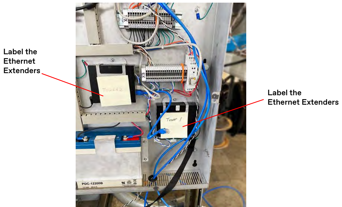
Figure 5 - Label and Wiring Overview
